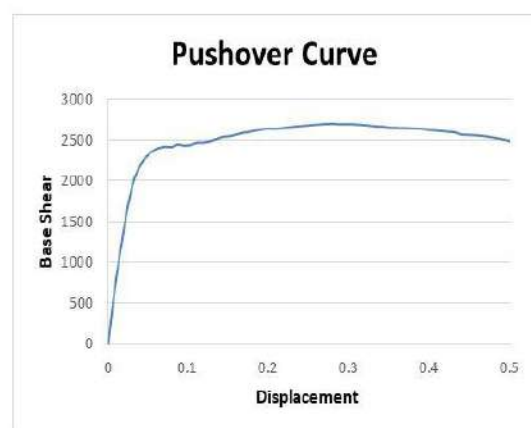
Figure 8: Push over curve for trapezoidal section
