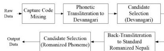
Figure 2. NEPTUN Normalization
