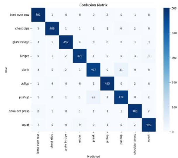
Figure 12. Confusion matrix
