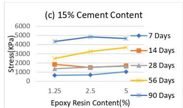
Figure 4: Plot of Unconfined Compressive Strength Vs Epoxy resin content for soil samples prepared with (a) 5% cement; (b) 10% cement; (c) 15% cement for five different curing periods
