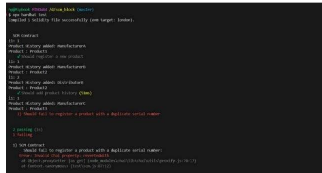
Figure 6. Testing Contracts Using Hardhat
