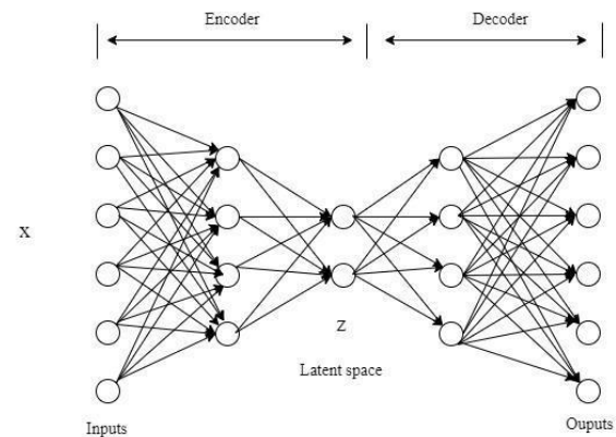
Figure 3. Fully Connected Autoencoders [10], [13]
